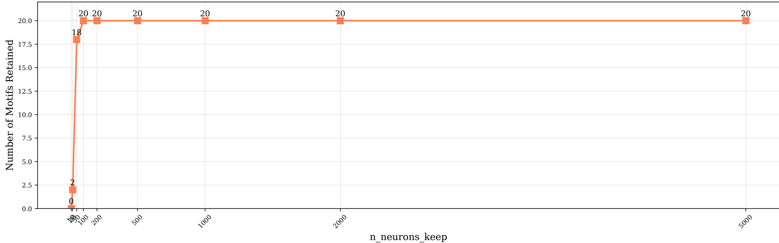
Motif Retention vs Neuron Threshold sigma: (0.02, 0.4) | volume: (0.05, 0.9)
